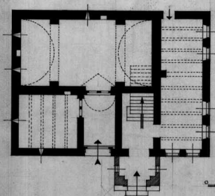
PLAN PARTER
